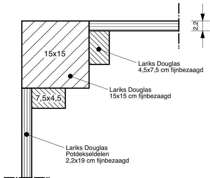
Detail 3
